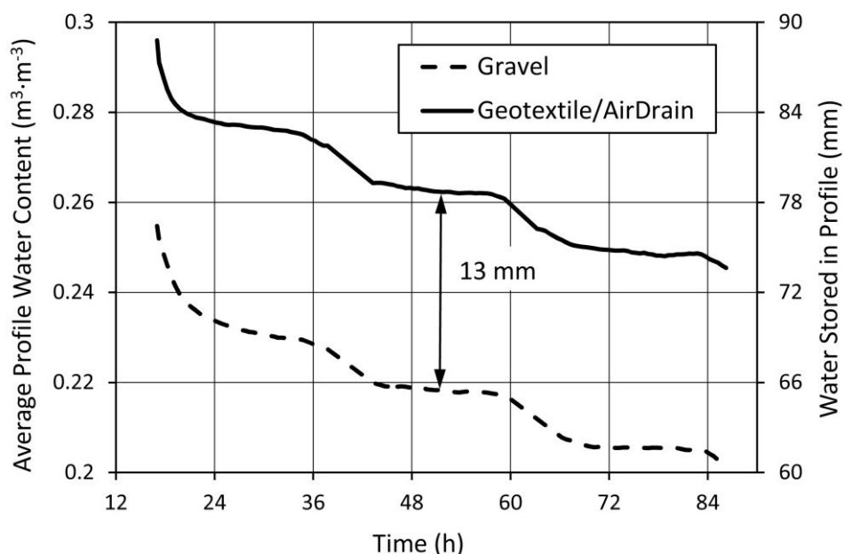
Figure 9. Temporal change in water stored in Sure Play root zone mixture atop gravel and atop geotextile/AirDrain in uncovered test greens. Stored water measured by vertical TDR probes. Water loss was by drainage and evapotranspiration. probes. Water loss was by drainage only.
