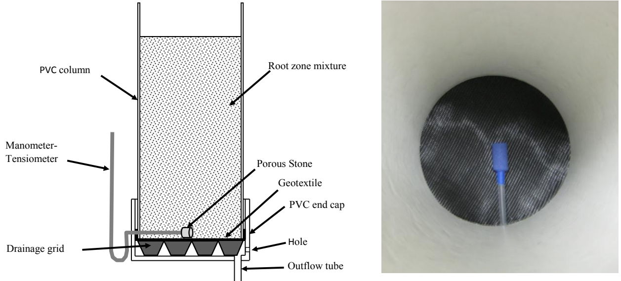
Figure 20. Schematic diagram of a longitudinal section of a test column (left). View into a test column showing a tensiometer-manometer atop a geotextile before the column was filled with root zone mixture (right).
