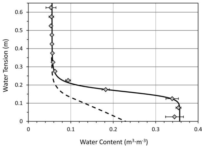
Figure 13. Relationship between water content and water tension for the root zone material. The solid line represents a curve fit of the model of Van Genuchten (1980). The dashed line represents the average water content of 0.3 m of root zone material above the location in the root zone having the given tension shown on the y-axis (e.g., if the bottom of a 0.3-m deep root zone were at 0.05 m tension, the average water content of the 0.3-m deep root zone would be about 0.18 \text{ m}^3 \cdot \text{m}^{-3} ).
