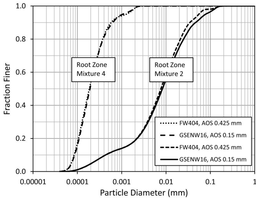
Figure 27. Size distribution of particles passing out of Root Zone Mixtures 2 and 4 and through the Geotextiles FW404 and GSEW16.
